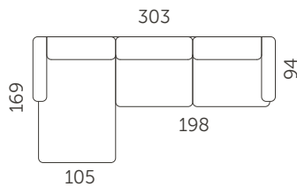
S72-1DML3CR
